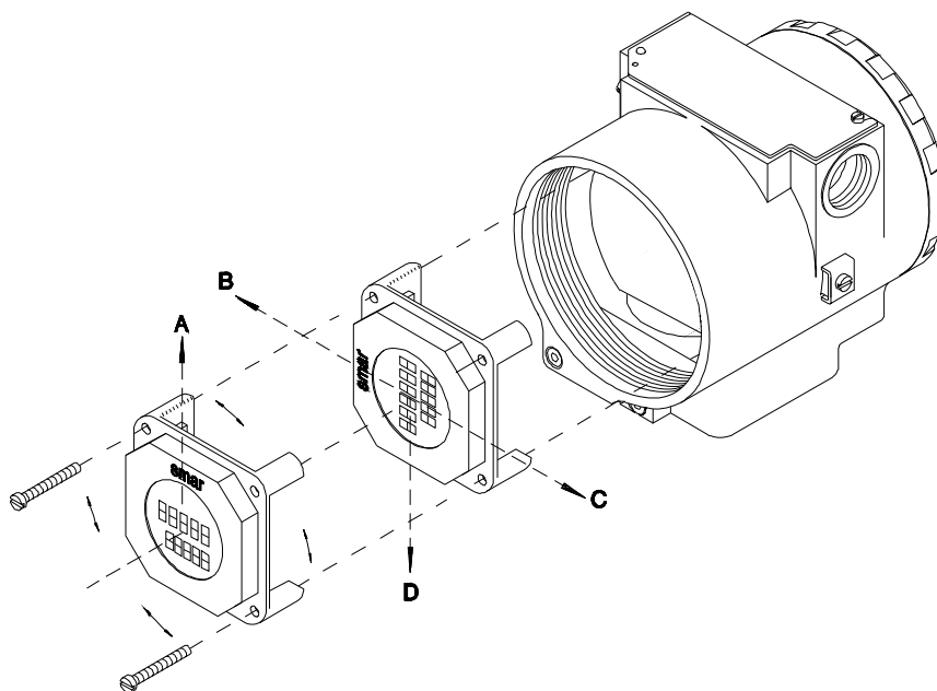
Figure 4.3 - Four Possible Positions of the Display
