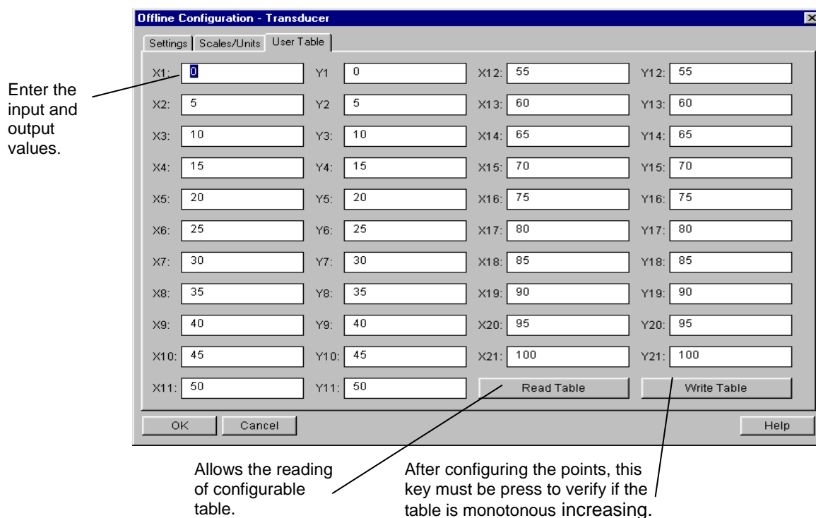
Figure 3.8 –Transducer Off Line Configuration – User Table Screen
