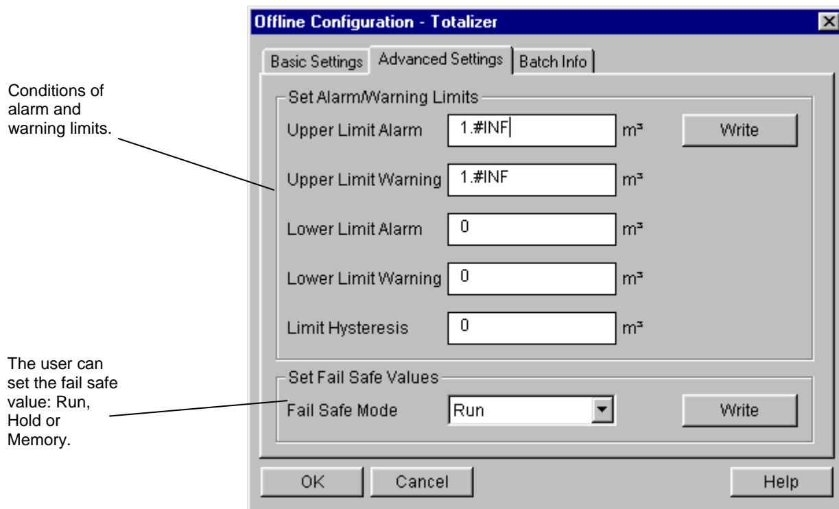
Figure 3.19 – Advanced Settings for Totalizer Block
