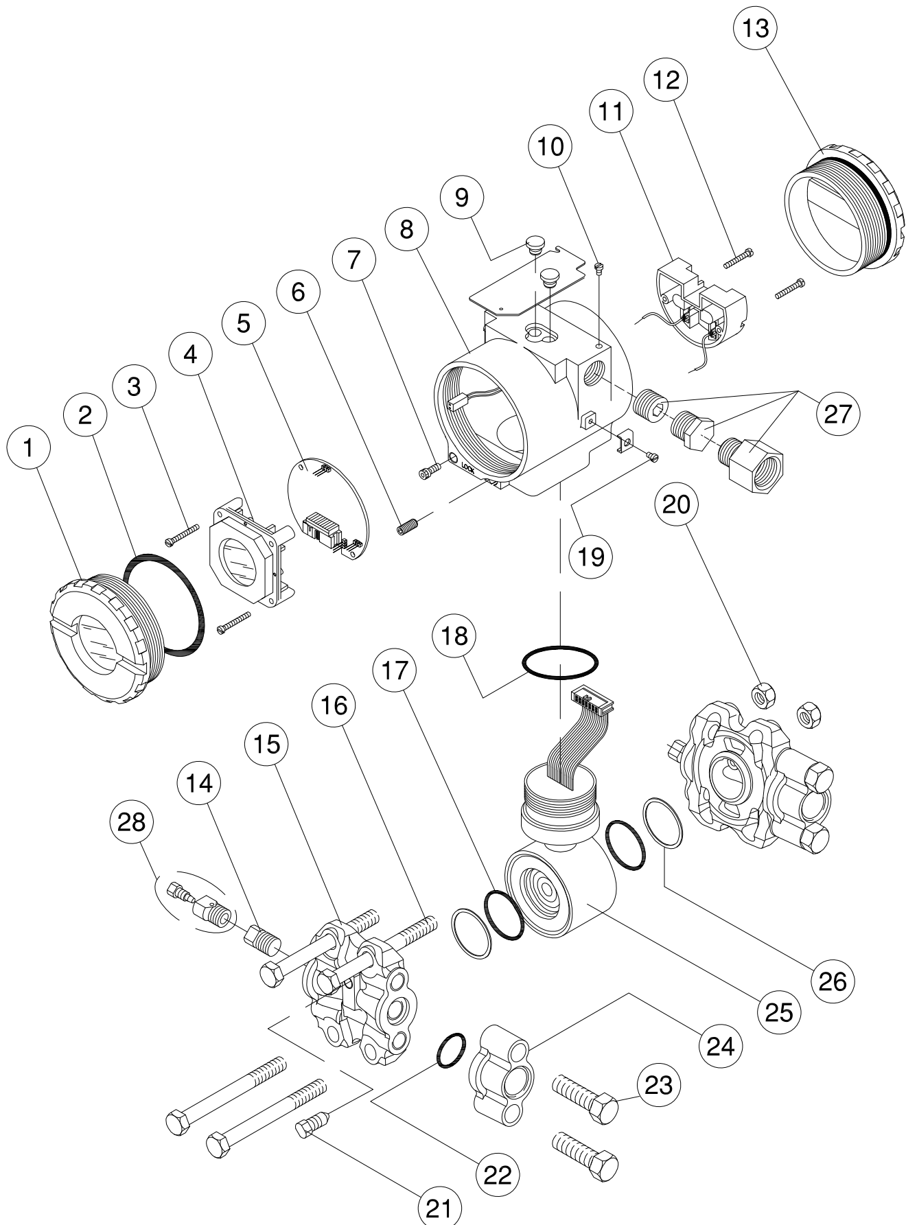
Figure 4.4 - Exploded View
