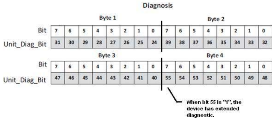
Figure 3.48 – Cyclic Diagnosis mapping for 4 bytes of Physical Block.
