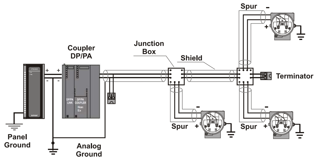
Figure 1.9 - Bus Topology
