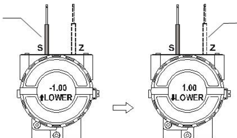
Figure 3.44 - Step 4 - LD303
