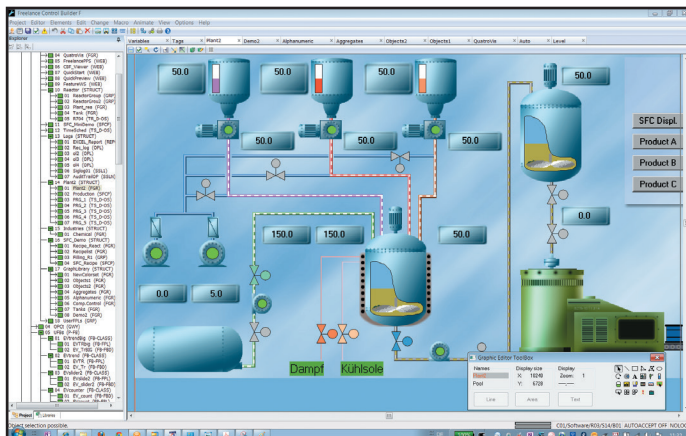
Graphics Editor
