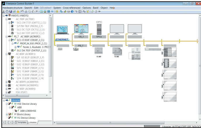
Definition of the hardware structure
