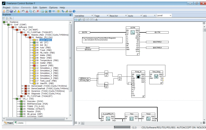
Project Tree with Function Block Diagram
