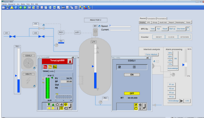
Graphic display with faceplates
