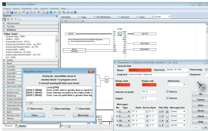
Program with parameterization screen and plausibility check
